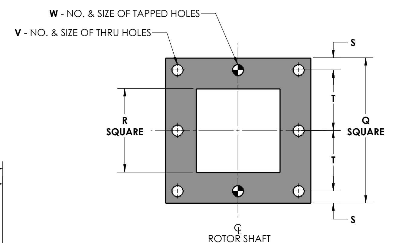
SQUARE FLANGE DETAIL (SEE NOTE # 2)
