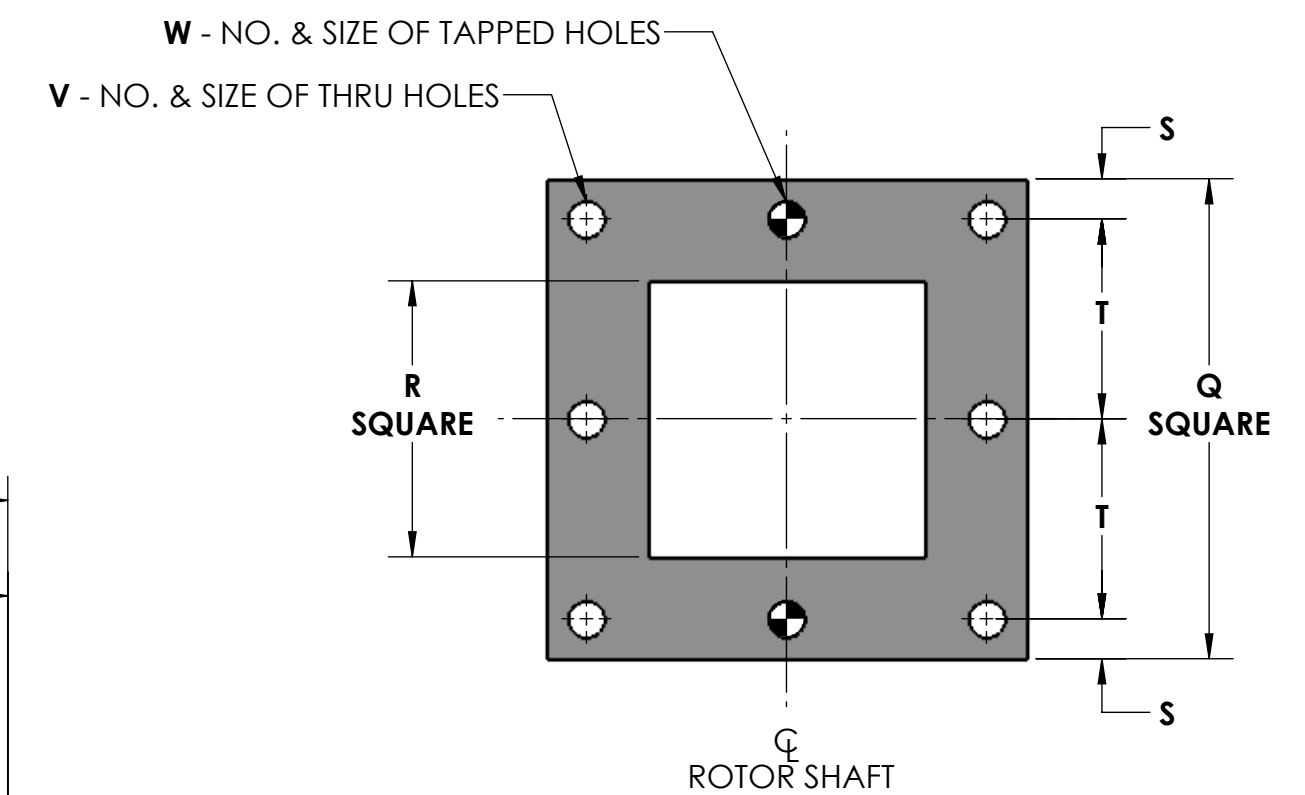
SQUARE FLANGE DETAIL (SEE NOTE # 2)
