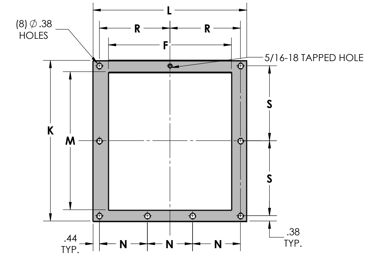
PRODUCT INLET FLANGE DETAIL
