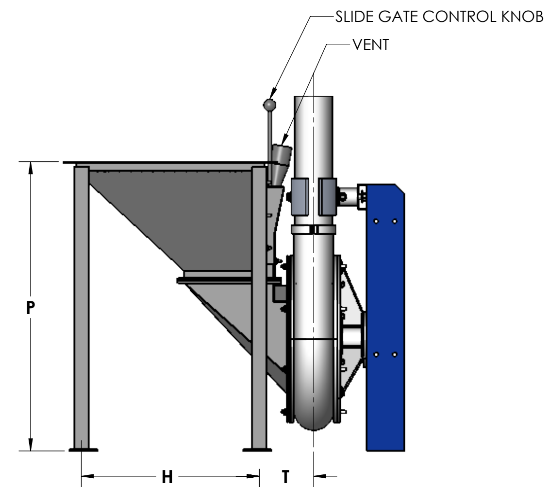
STANDARD CHARGE HOPPER DETAIL 1.50 CU. FT. CAPACITY (OPTIONAL)
