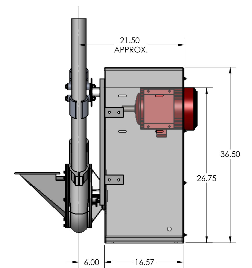
BOTTOM DRIVE DETAIL (OPTIONAL)
